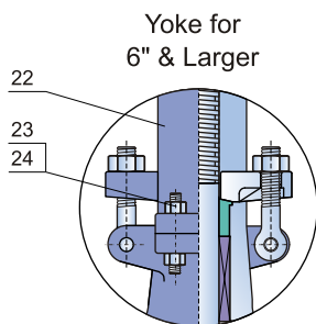
Yoke for 6" & Larger
