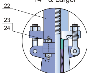
Yoke for 14" & Larger
