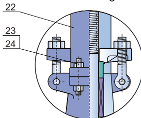
Yoke for 12" &amp; Larger
