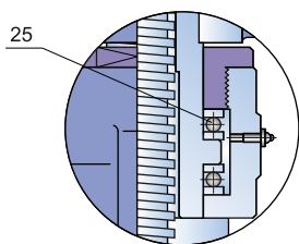
Bearing for 6" &amp; Larger
