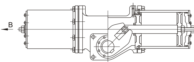
View A
