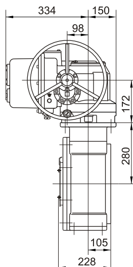
Overall Dimensions &amp; Weight of Electric Actuator
