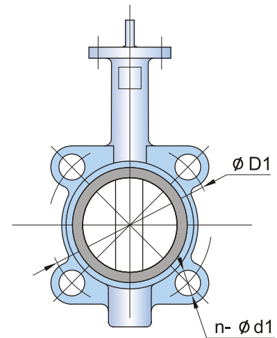
WAFER TYPE Series 300W
