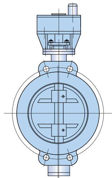
WAFER/LUG TYPE
